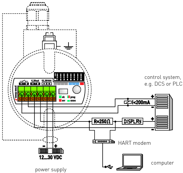
Figure 6: electrical connection
