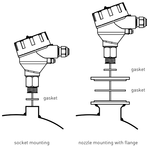
Figure 4: mounting
