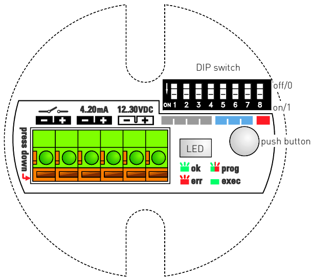
Figure 9: control elements
