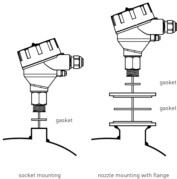
Figure 1: mounting
