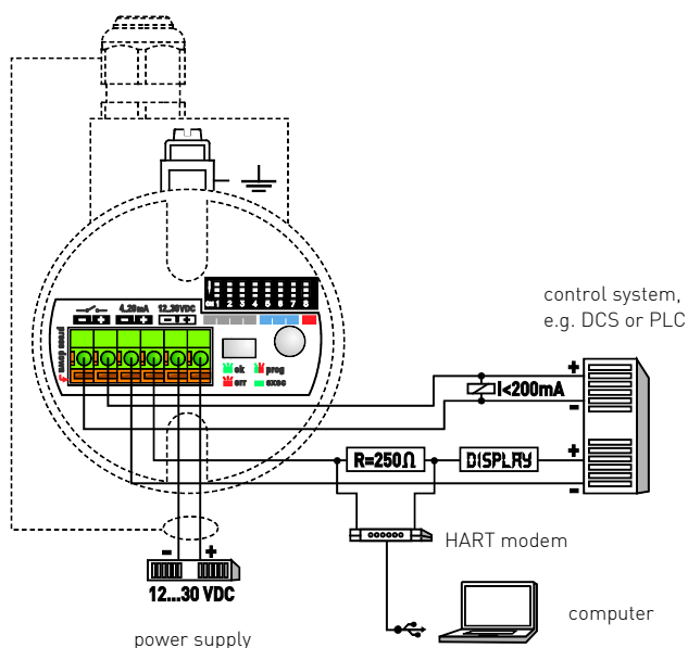
Figure 8: wiring
